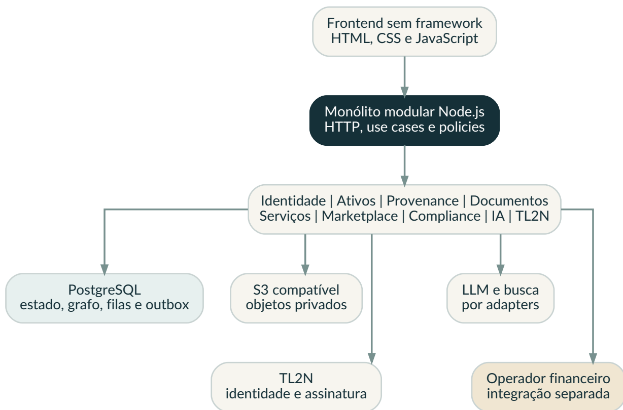
Logical architecture
